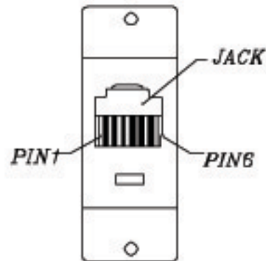
RJ12 JACK
